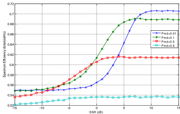
Figure 3. Spectrum efficiency vs. SNR considering sensing errors
