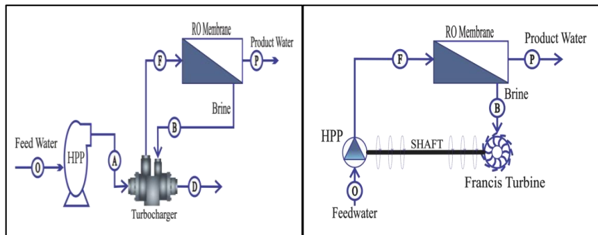
Figure 4. Scheme of the Francis Turbine and Turbocharger in the plant.
