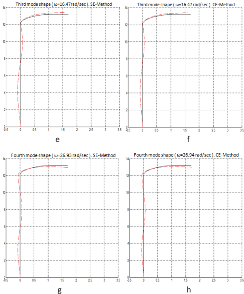
Figure (6): Comparison the third and the forth mode shapes of the lighting column from the SE and CE finite element methods.
