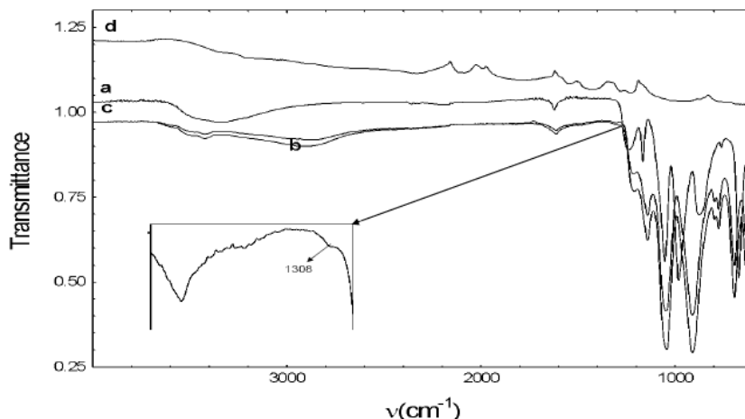
Figure 2. FT-IR spectra of: (a) pure JDF-L1; (b) polyaniline-JDF-L1 (13.4 wt% PANI) nanocomposite; (c) polyaniline-JDF-L1 (8.7 wt% PANI) nanocomposite; (d) pure polyaniline
