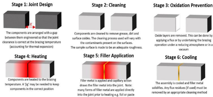
Figure 6. Brazing joining process
