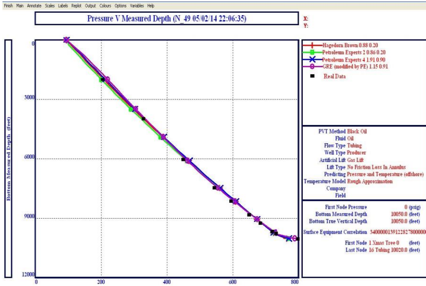
Figure 10: Pressure gradient of Well N49 Using Software
