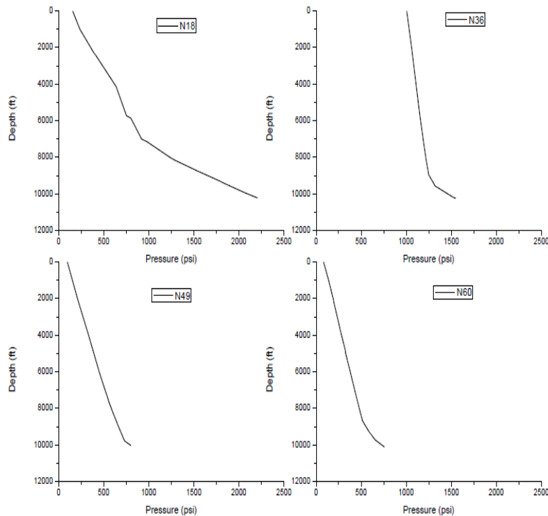
Figure 5: Pressure Gradient of all Wells
