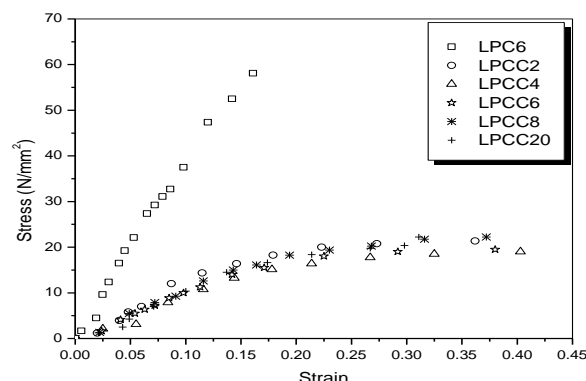
Figure 3. Stress-strain curves of LLDPE/CKD composites containing 6 wt% of CKD with various CO contents.
